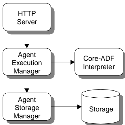
Figure 1. The Agent Server Architecture
