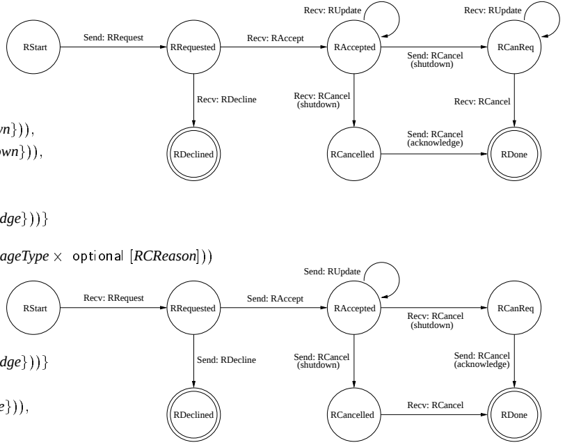
Figure 1. Registration Requestor and Provider Protocols
