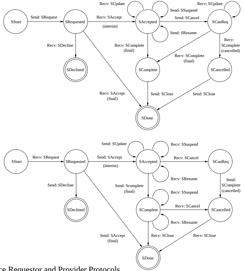
Figure 2. Service Requestor and Provider Protocols
